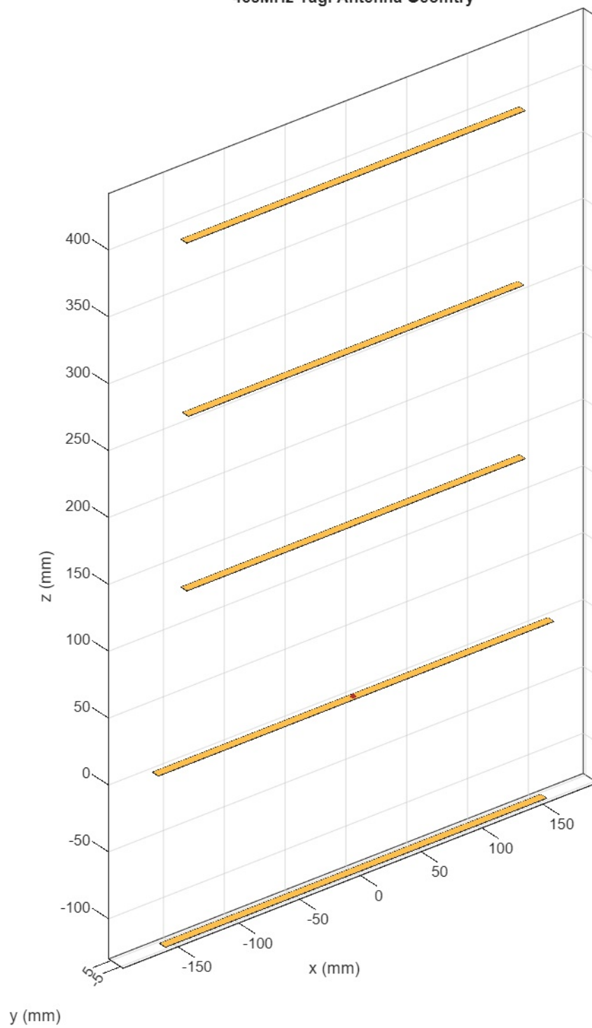
435MHz Yagi Antenna Geomtry
